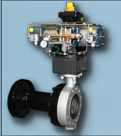
ANSI 600# Triple Offset Metal Seated Isolation Valve with Automation & Spool for drop in replacement of lift & turn ball valve
